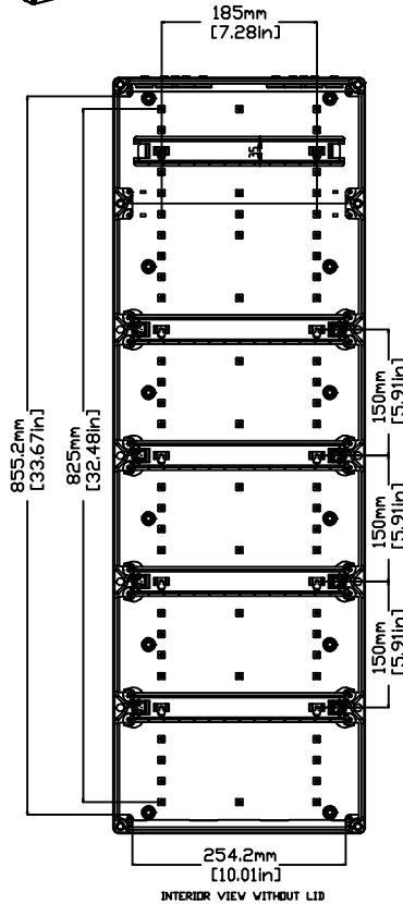
INTERIOR VIEW WITHOUT LID
