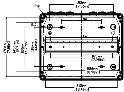
INTERIOR VIEW WITHOUT LID
