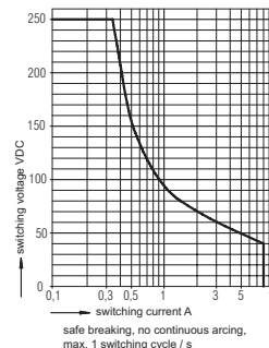
Maximum switching power curve Limit curve for arc-free operation safe breaking, no continuous arcing, max. 1 switching cycle / s
