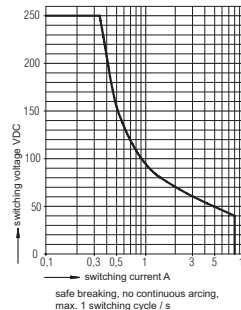
Maximum switching power curve safe breaking, no continuous arcing, max. 1 switching cycle / s
