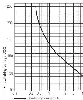
Maximum switching power curve safe breaking, no continuous arcing, max. 1 switching cycle / s
