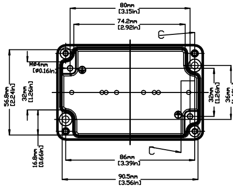
TOP VIEW WITHOUT LID
