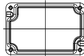
INTERIOR VIEW OF LID
