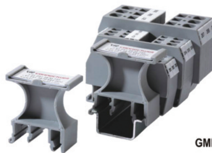
Mountable on All mounting rails Dimension GMH6 46.5(H) x 44.5(W) x 9.5(T) mm
