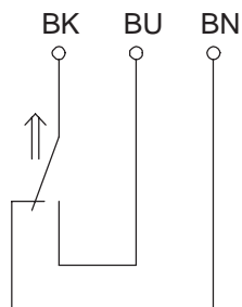
Wiring diagram ( matching to the drawing )
