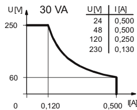
Performance diagram
