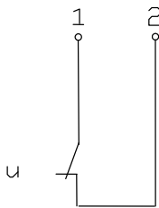
Wiring diagram (non-actuated state)
